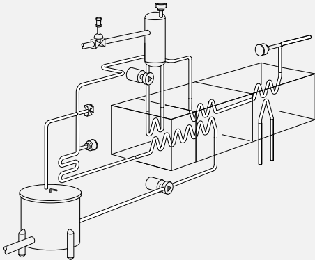
Pasteurising plant
