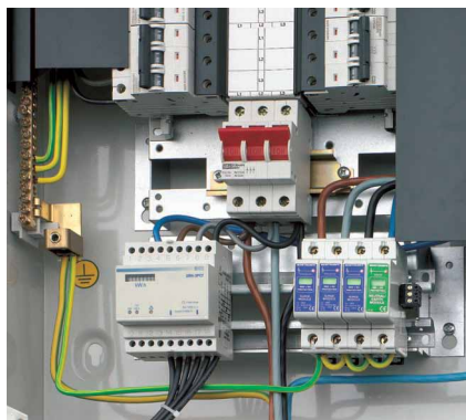
Typical Distribution Board
